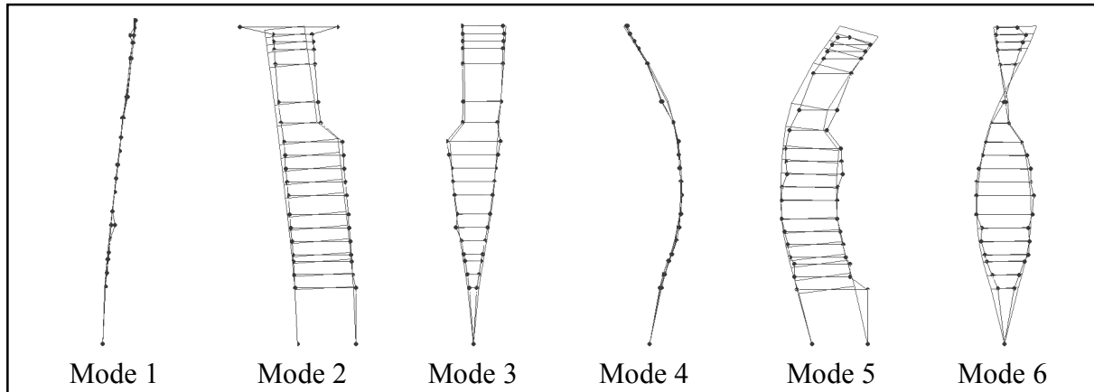
Figure 3. EMA and FEM shapes after updating.
