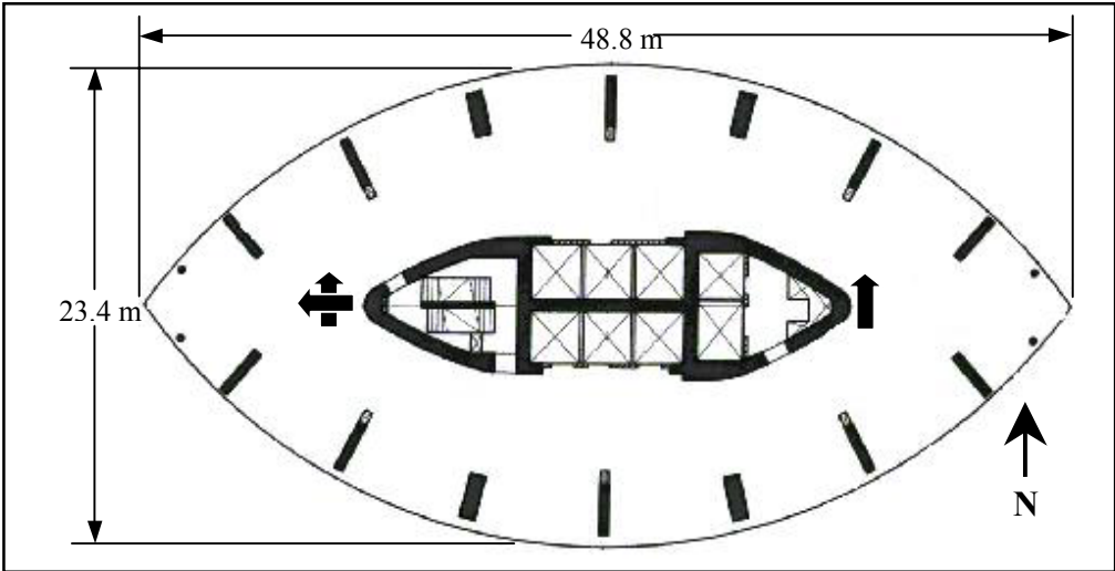
Figure 2. Typical floor plan and sensor location.
